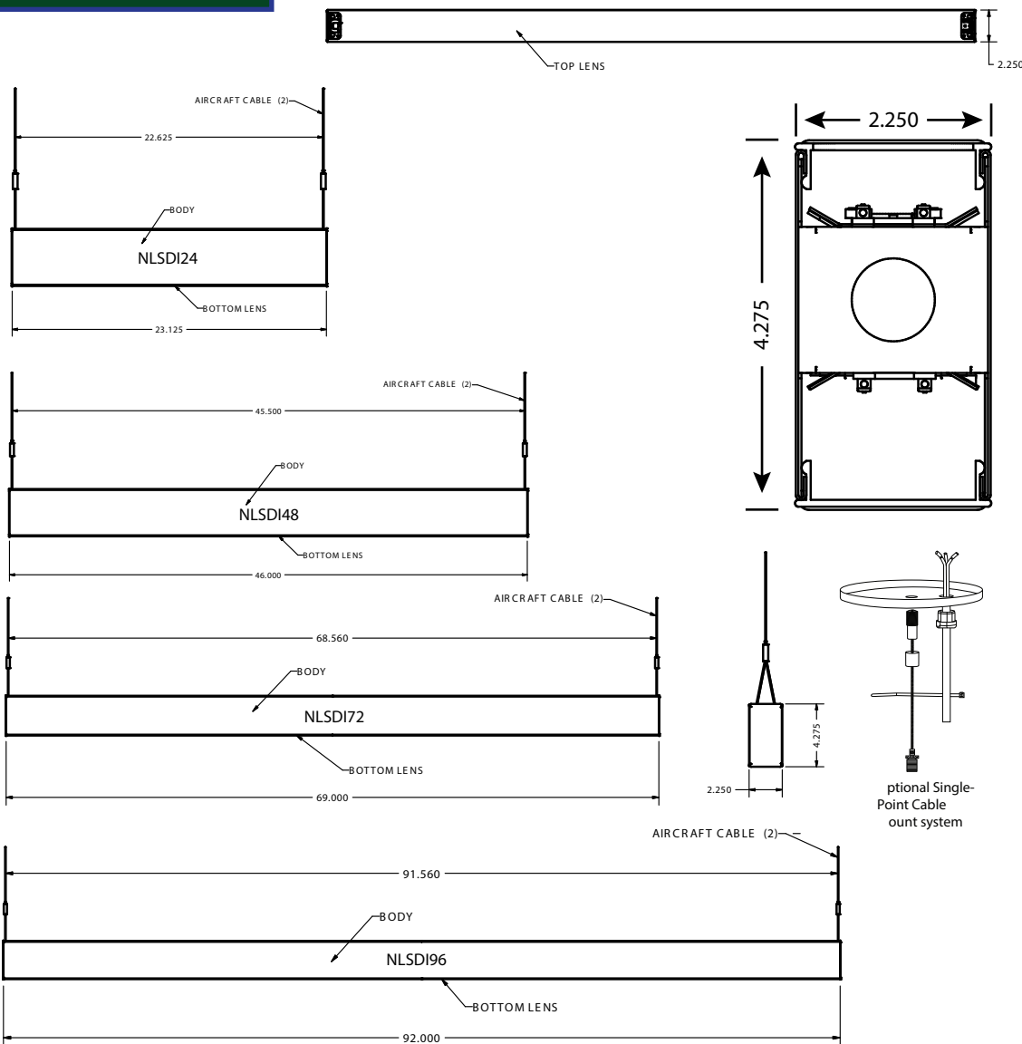
Cable Mounting Detail
